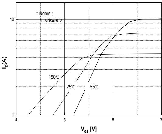
Fig.5 Transfer Characteristics
